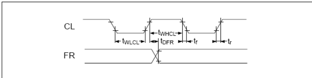
Figure 3: Control Timing Waveform
