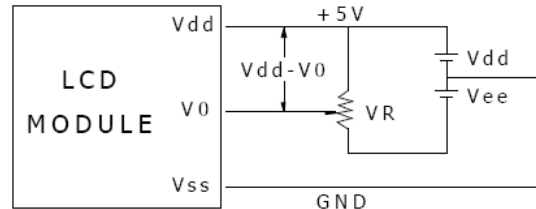
Vdd-V0: LCD Driving Voltage VR: 10K - 20K
